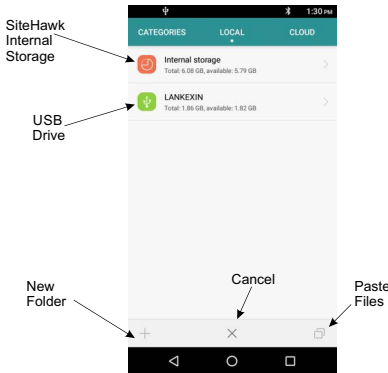
Figure 41 Paste Files
