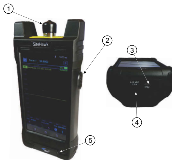
Figure 1 SK-6000 Controls, Indicators, Connectors and Ports
