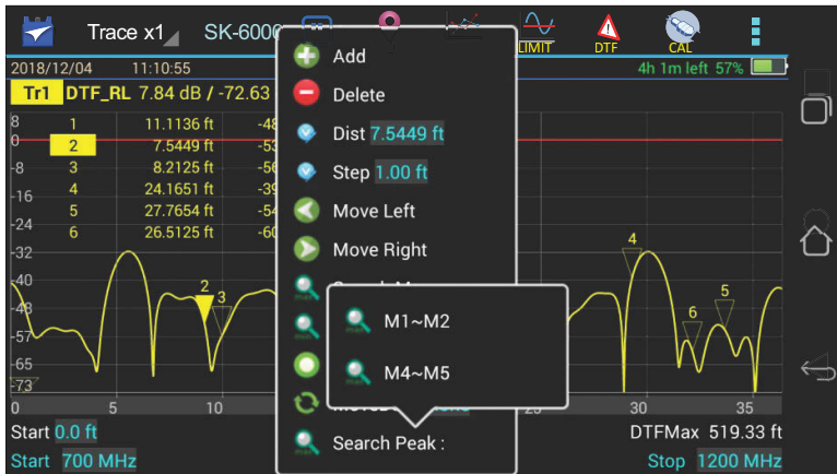
Figure 16 Marker Menu
